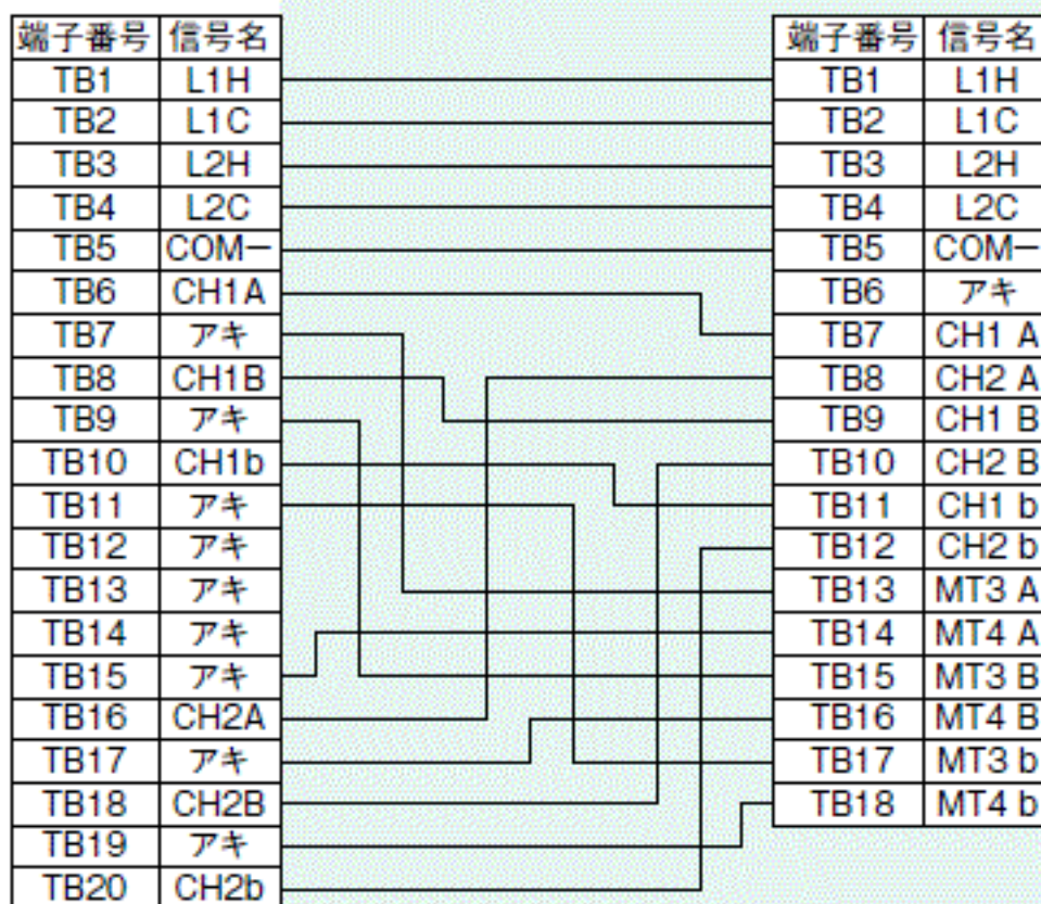
A1S62TCRT-S2 端子台
